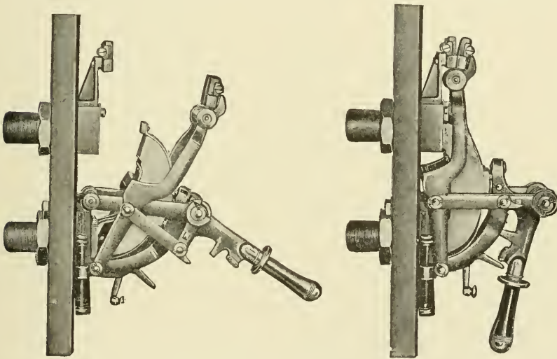
Fig. 152. General Electric Circuit Breaker
